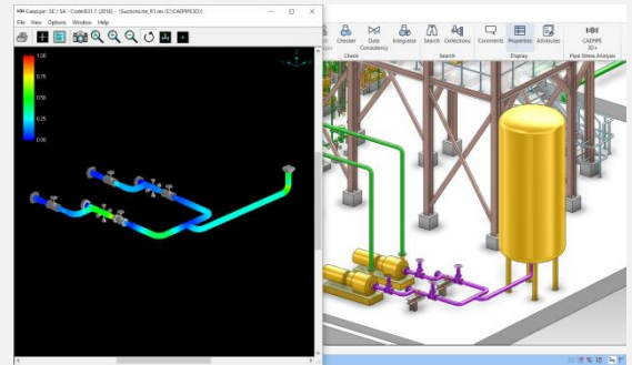
First-level Stress Check on Revised Layout by Designer
