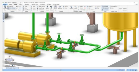
Finalized Layout & Supports transferred to 3D Plant by Designer
