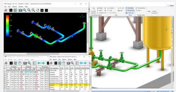
Detailed Analysis by Stress Engineer with 3D Plant Model in view
