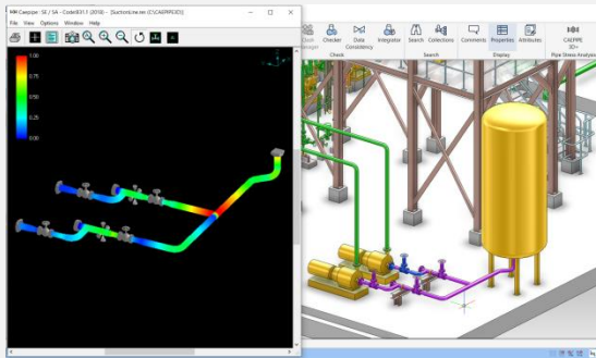
First-level Stress Check on Original Layout by Designer
