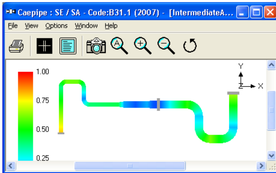
Figure 2E - Thermal Stress Contour Plot for Layout with Intermediate Anchor
