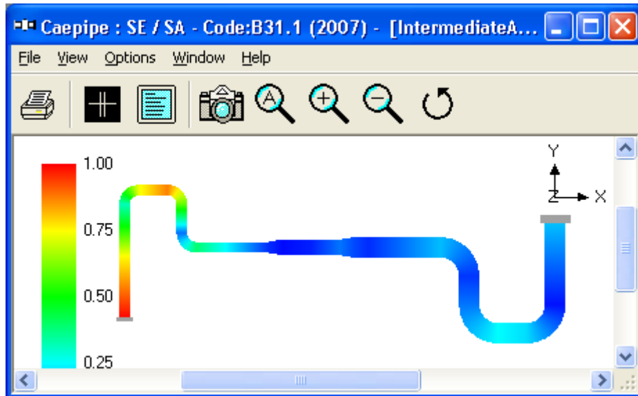
Figure 2C - Thermal Stress Contour Plot
