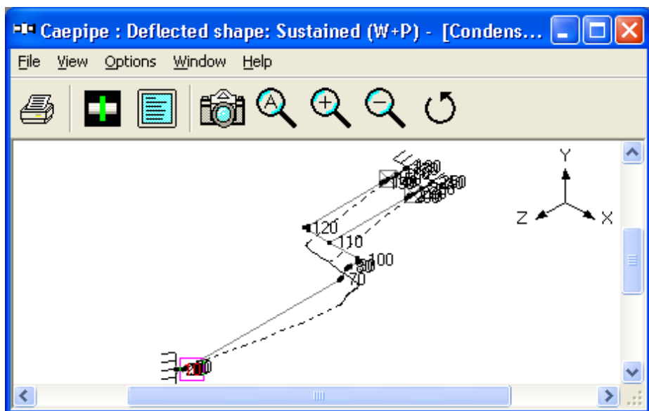
Figure 5B - Thermal Deformation Plot
