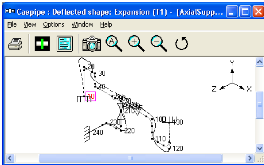
Figure 3E - Thermal Deformation Plot for Layout with Axial Restraints
