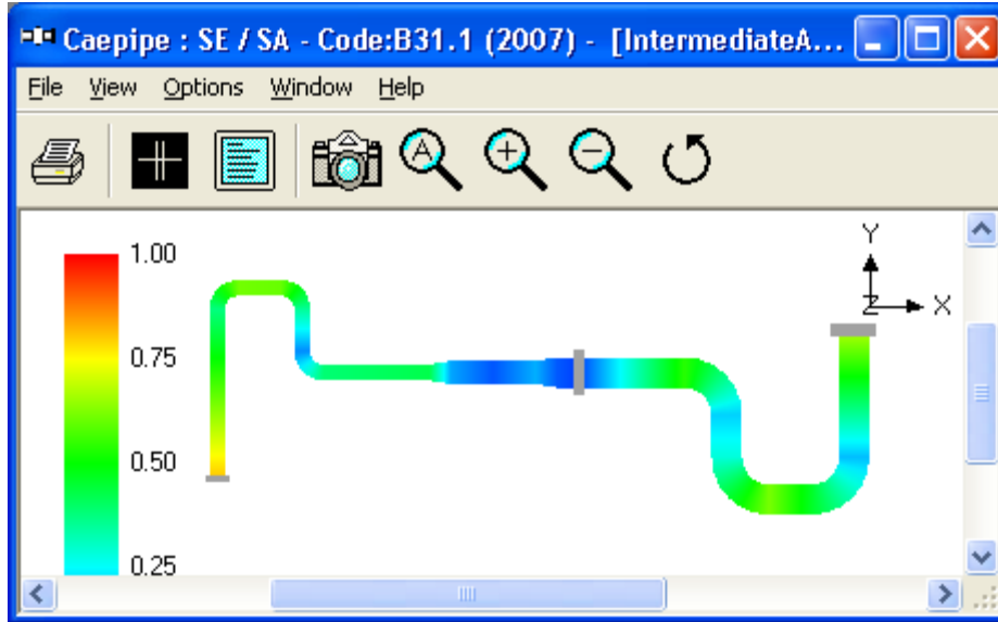
Figure 3A - Layout with Intermediate Anchor at Node 95
