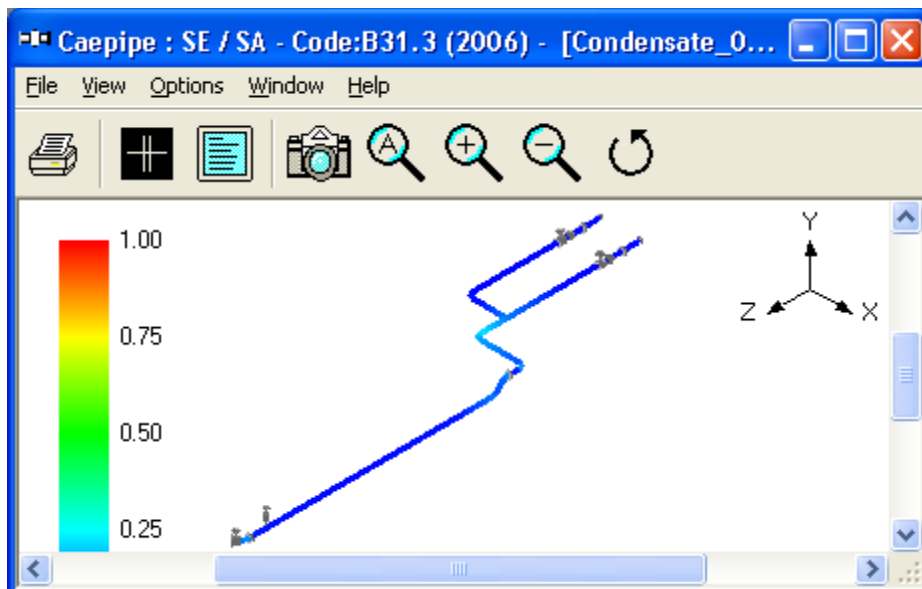
Figure 5F - Thermal Stress Contour Plot for Revised Layout
