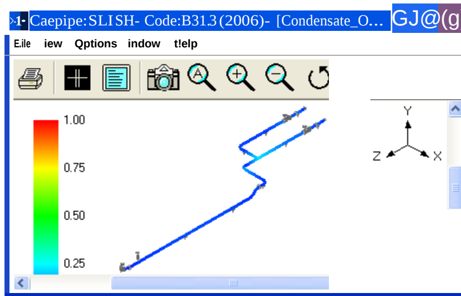
Figure 51- 9Jslaine::l Stress Contour Plot for Re-.tse::l layout Wth Resting SUpports
