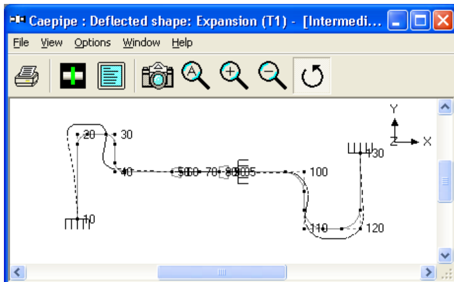
Figure 2D - Thermal Deformation Plot for Layout with Intermediate Anchor
