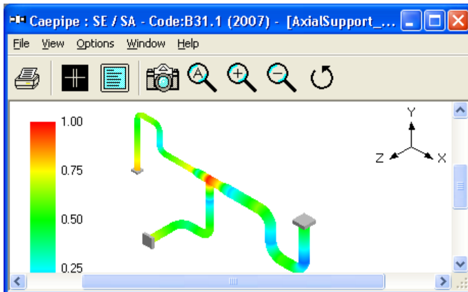
Figure 3F - Thermal Stress Contour Plot for Layout with Axial Restraints
