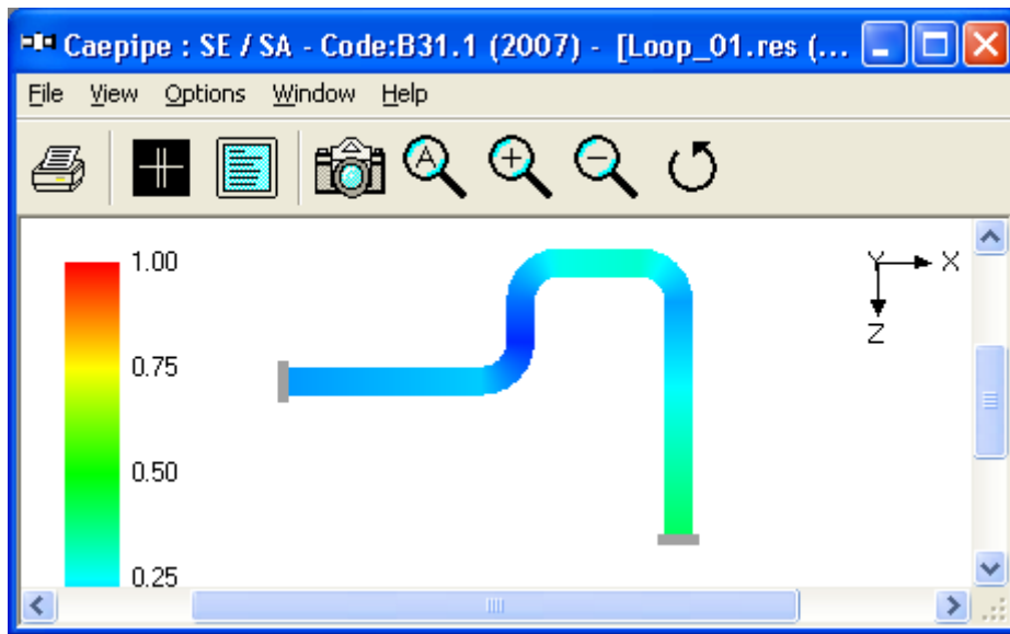
Figure 1F - Code-compliant sustained case
