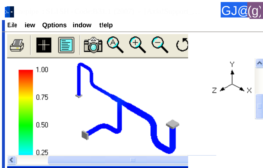
Figure 3G. SUSlaine::I Stress Contour Plot for layout Wth .Axial Restraints
