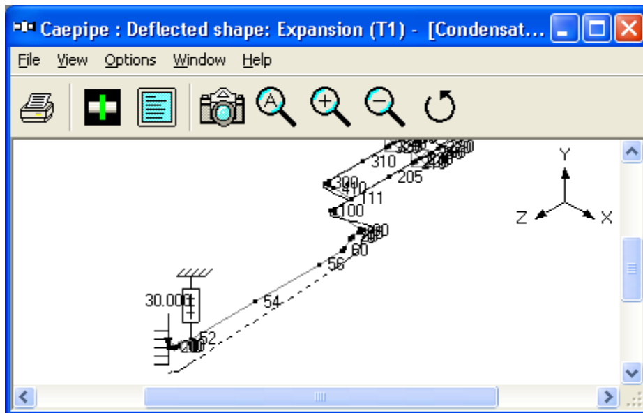
Figure 5E - Thermal Deformation Plot for Revised Layout
