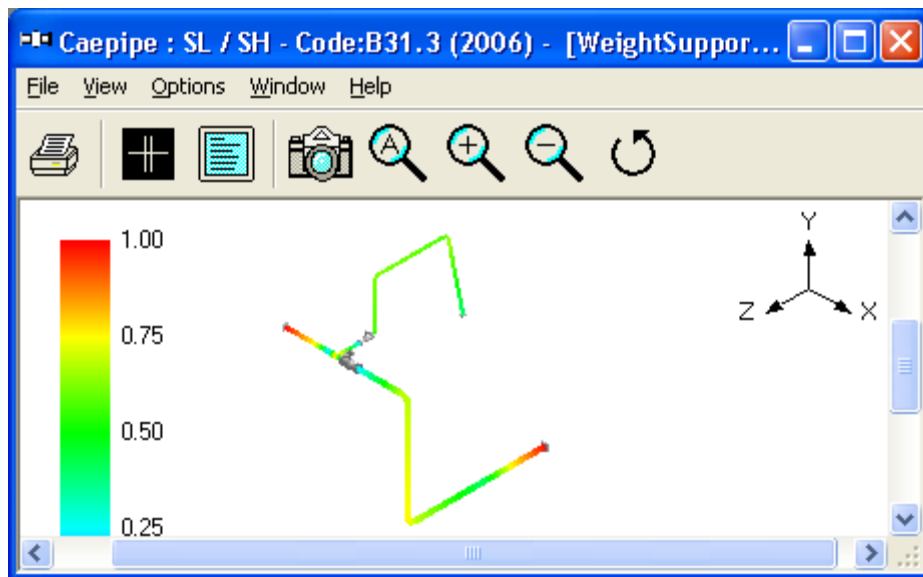
Figure 4D - Sustained Stress Contour Plot
