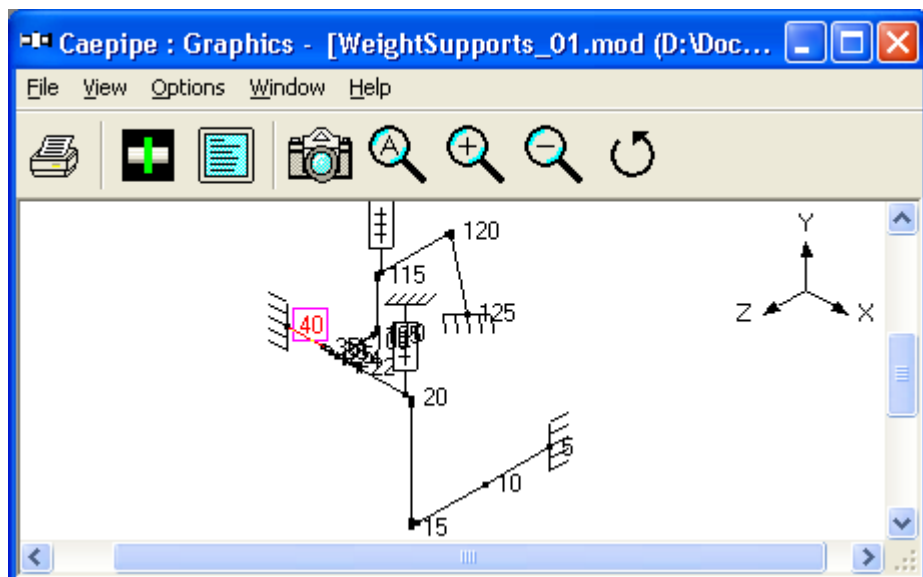
Figure 4E - Layout with Hangers
