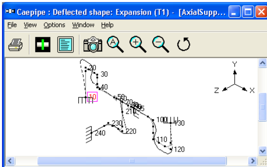
Figure 3B - Thermal Deformation Plot
