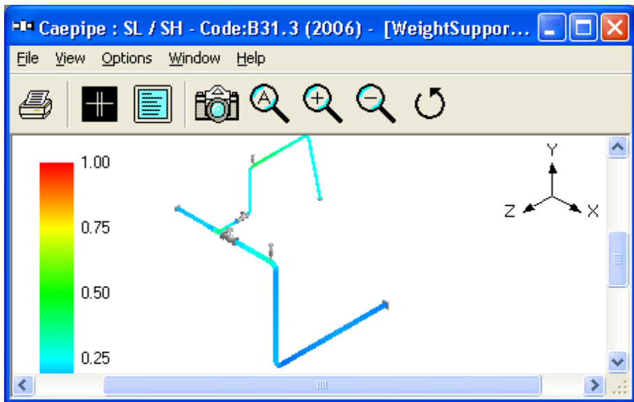
Figure 4G - Sustained Stress Contour Plot for Layout with Hangers
