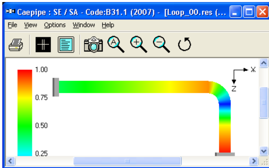
Figure 1C - Non code-compliant (notice the reds)
