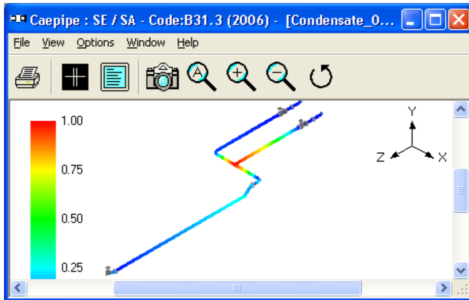
Figure 5C - Thermal Stress Contour Plot
