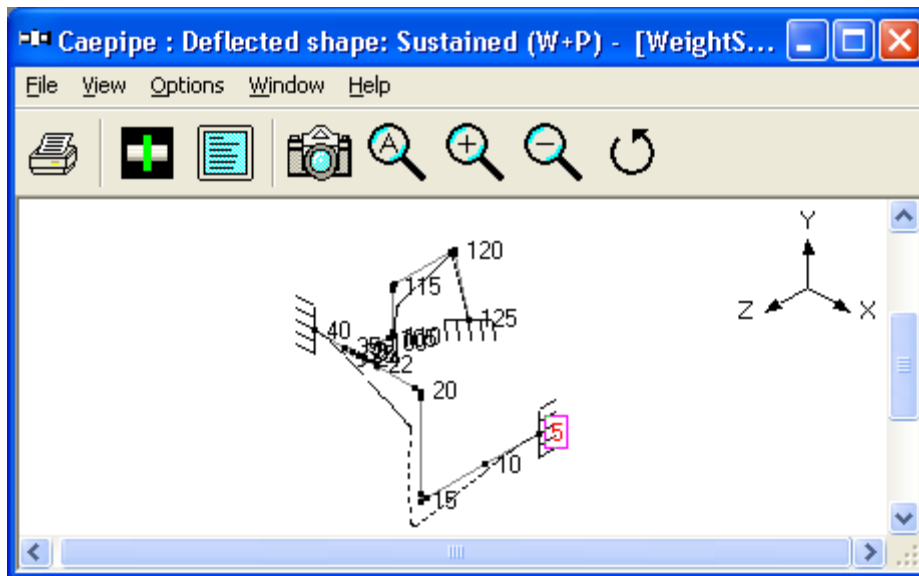
Figure 4C - Sustained Load Deflected Shape
