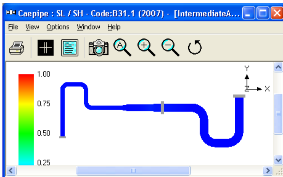
Figure 2F - Sustained Stress Contour Plot for Layout with Intermediate Anchor
