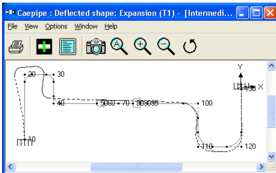
Figure 2B - Thermal Deformation Plot
