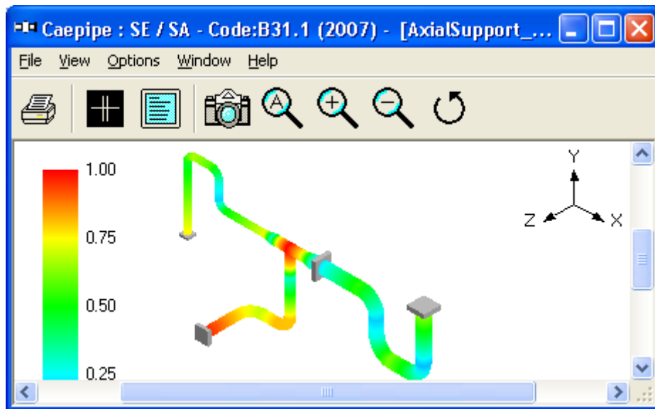
Figure 3D - Layout with Axial Restraints at Node 95 and 210
