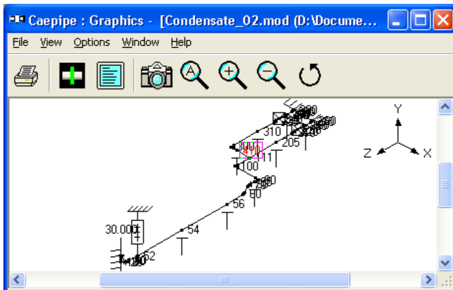
Figure 5H - Revised Layout with Resting Supports
