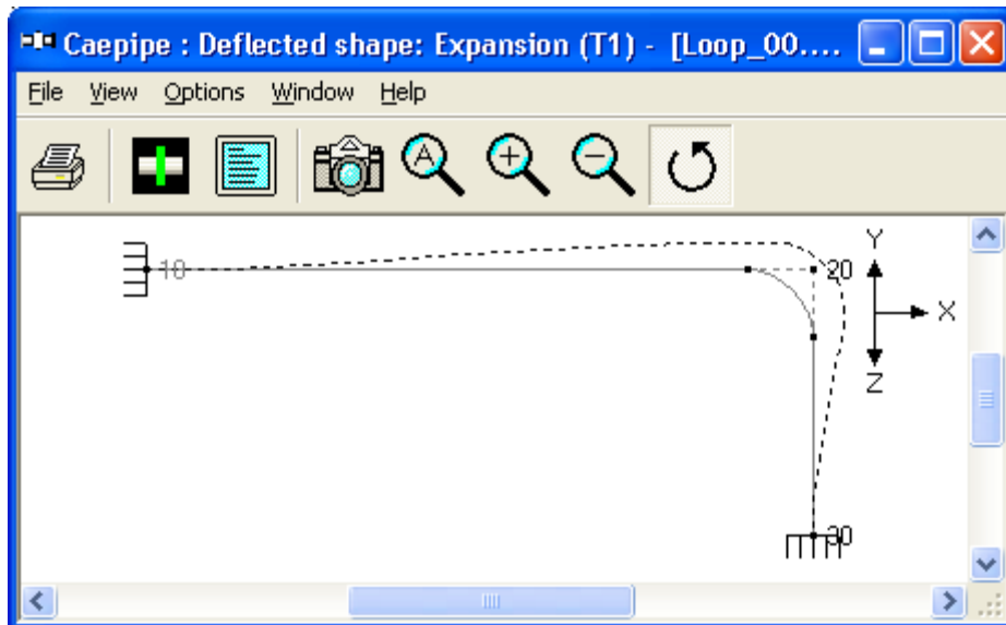
Figure 1B - Thermal Deflection
