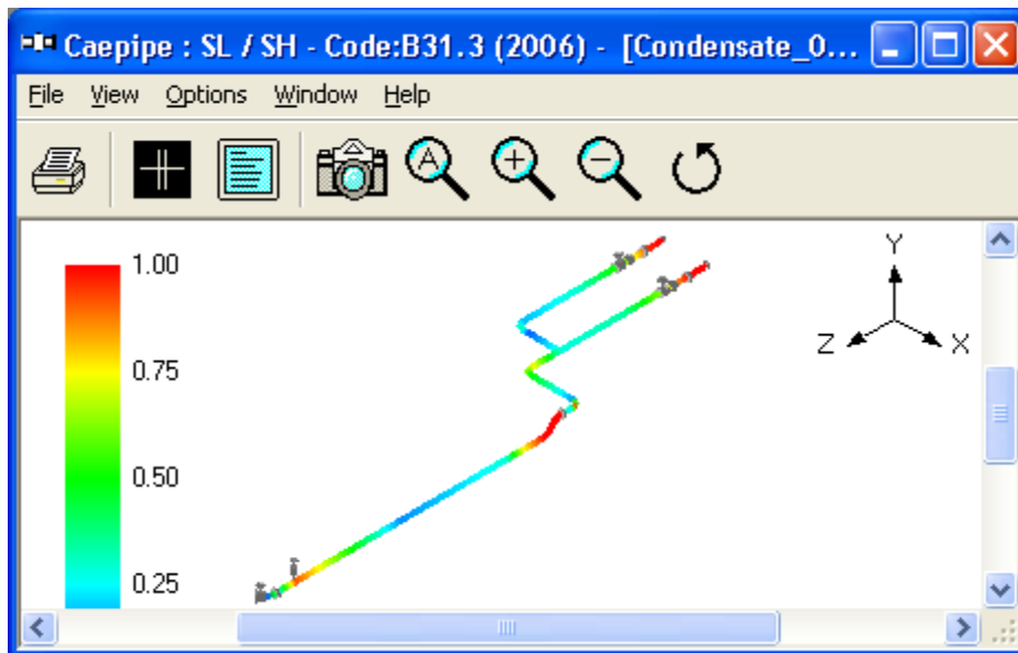
Figure 5G - Sustained Stress Contour Plot for Revised Layout
